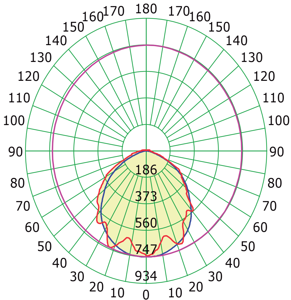
Luminous Intensity Distribution Curve
